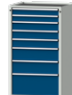
8 Schubladen 90, 90, 120, 120, 180, 180, 300 mm
